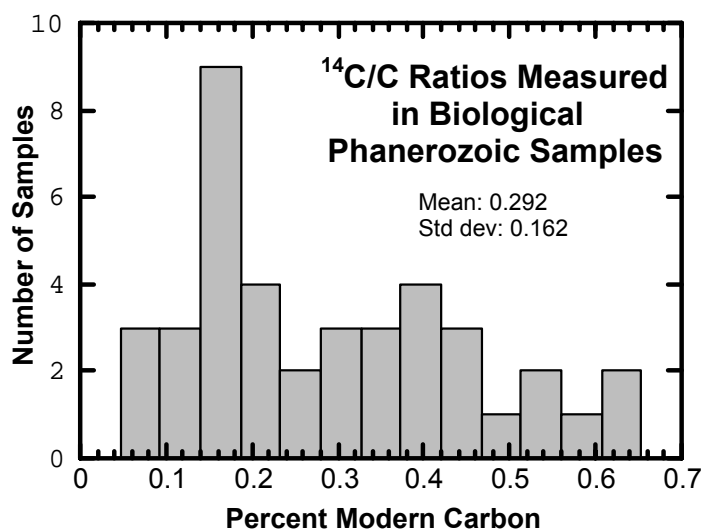
Figure 7. Distribution of ^{14}\text{C} values for biogenic samples from the radiocarbon literature. Given their position in the geological record, all these samples should contain no detectable ^{14}\text{C} according to the conventional geological time scale.
